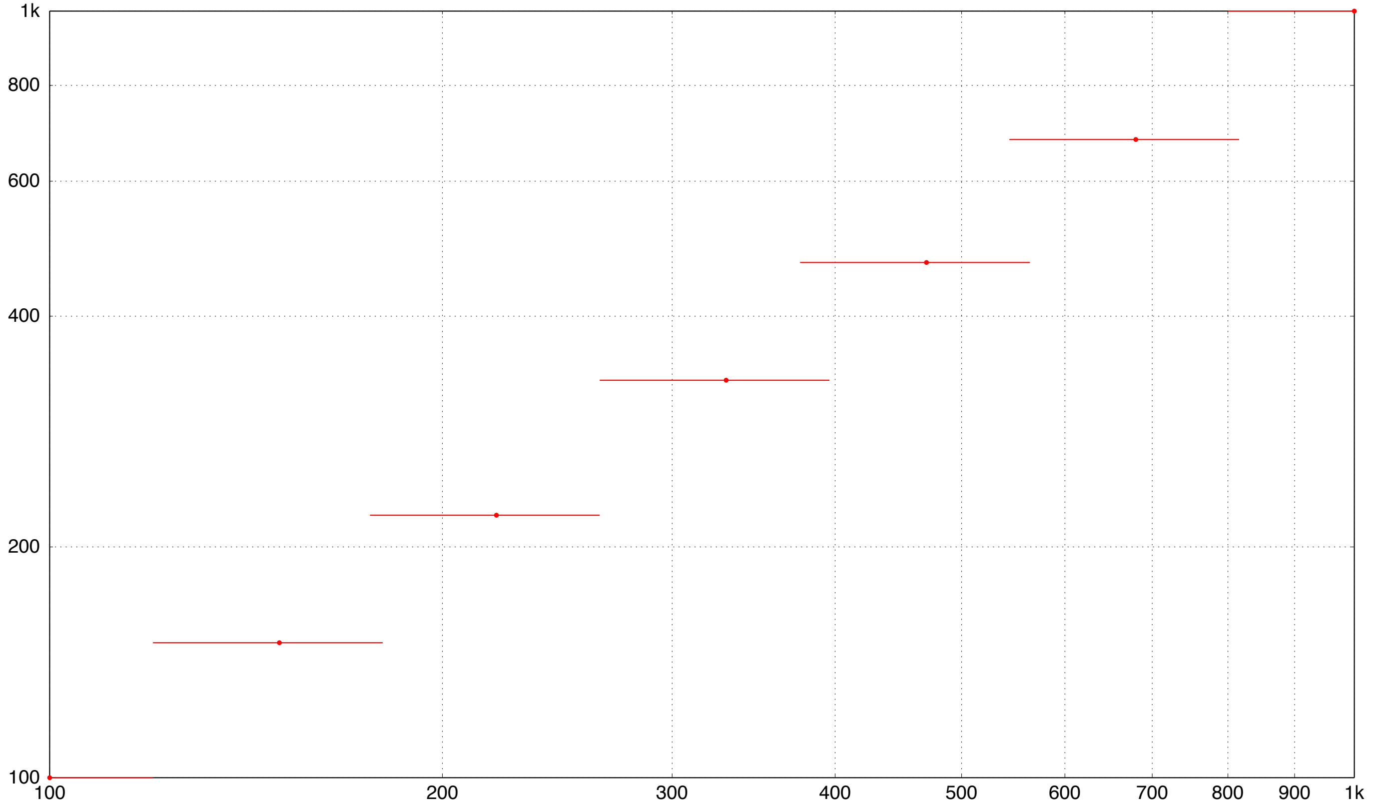
E6 series values between 100 and 1k with \pm 20\% tolerance bands
