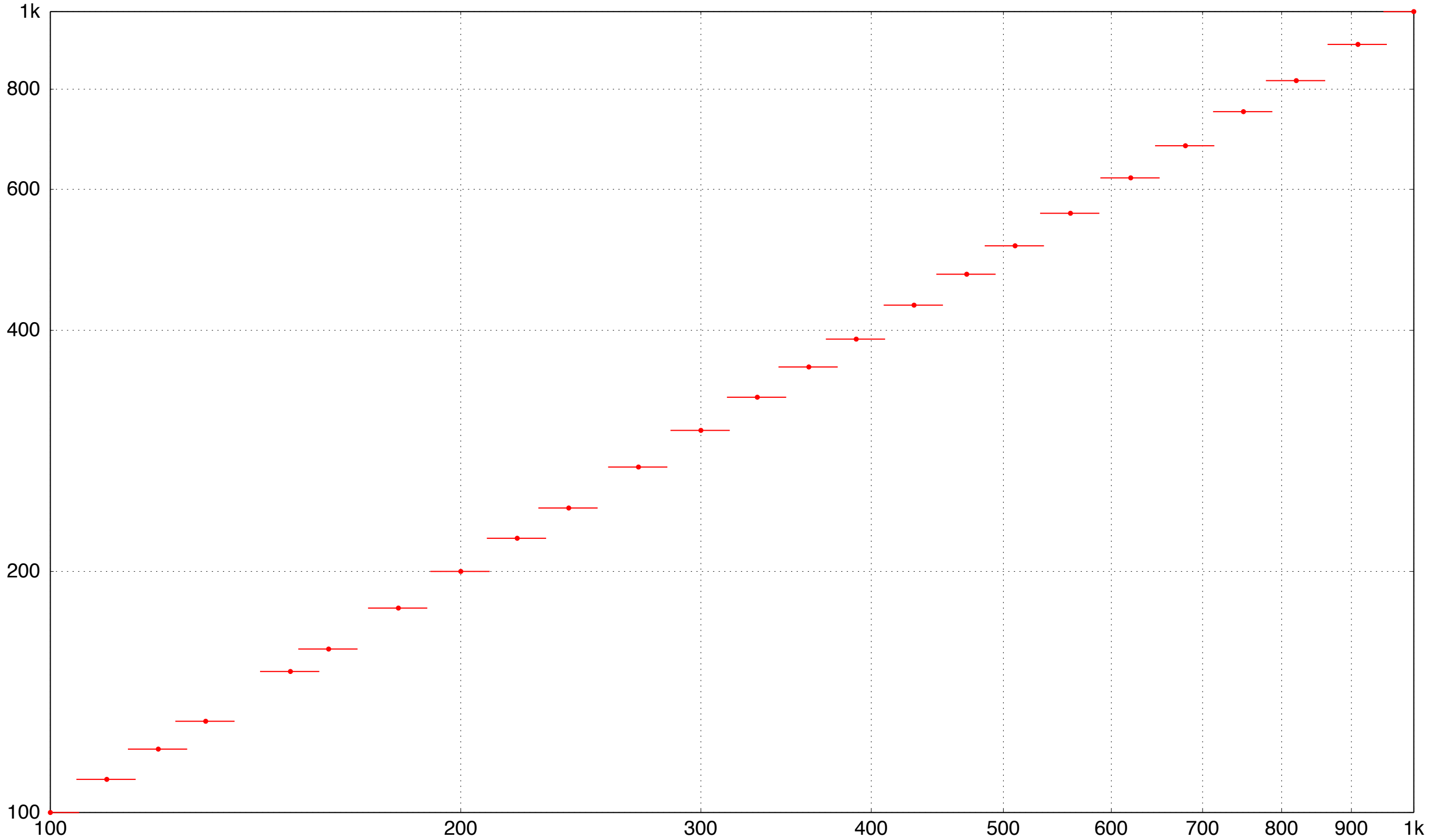
E24 series values between 100 and 1k with \pm 5\% tolerance bands
