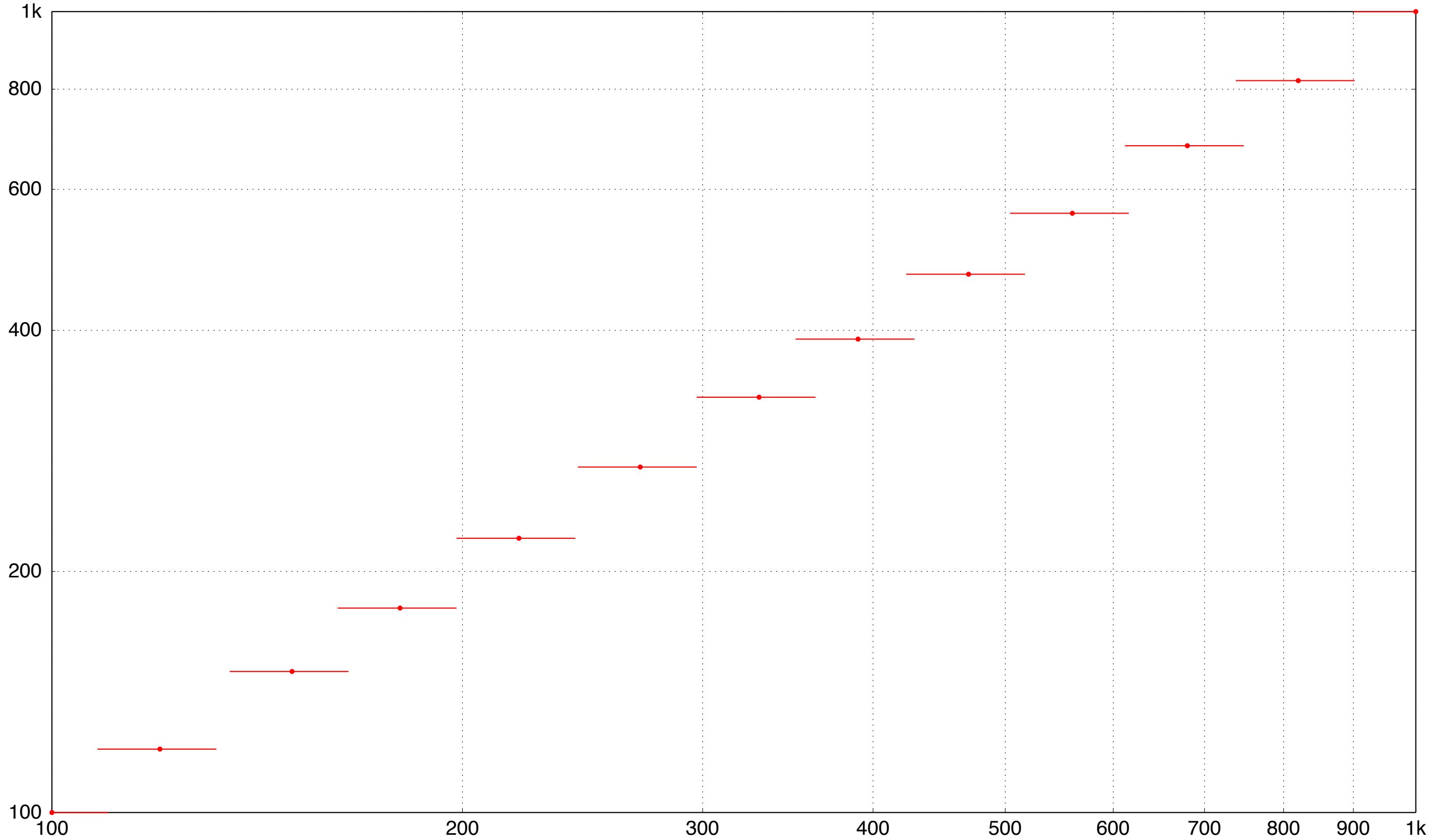
E12 series values between 100 and 1k with \pm 10\% tolerance bands
