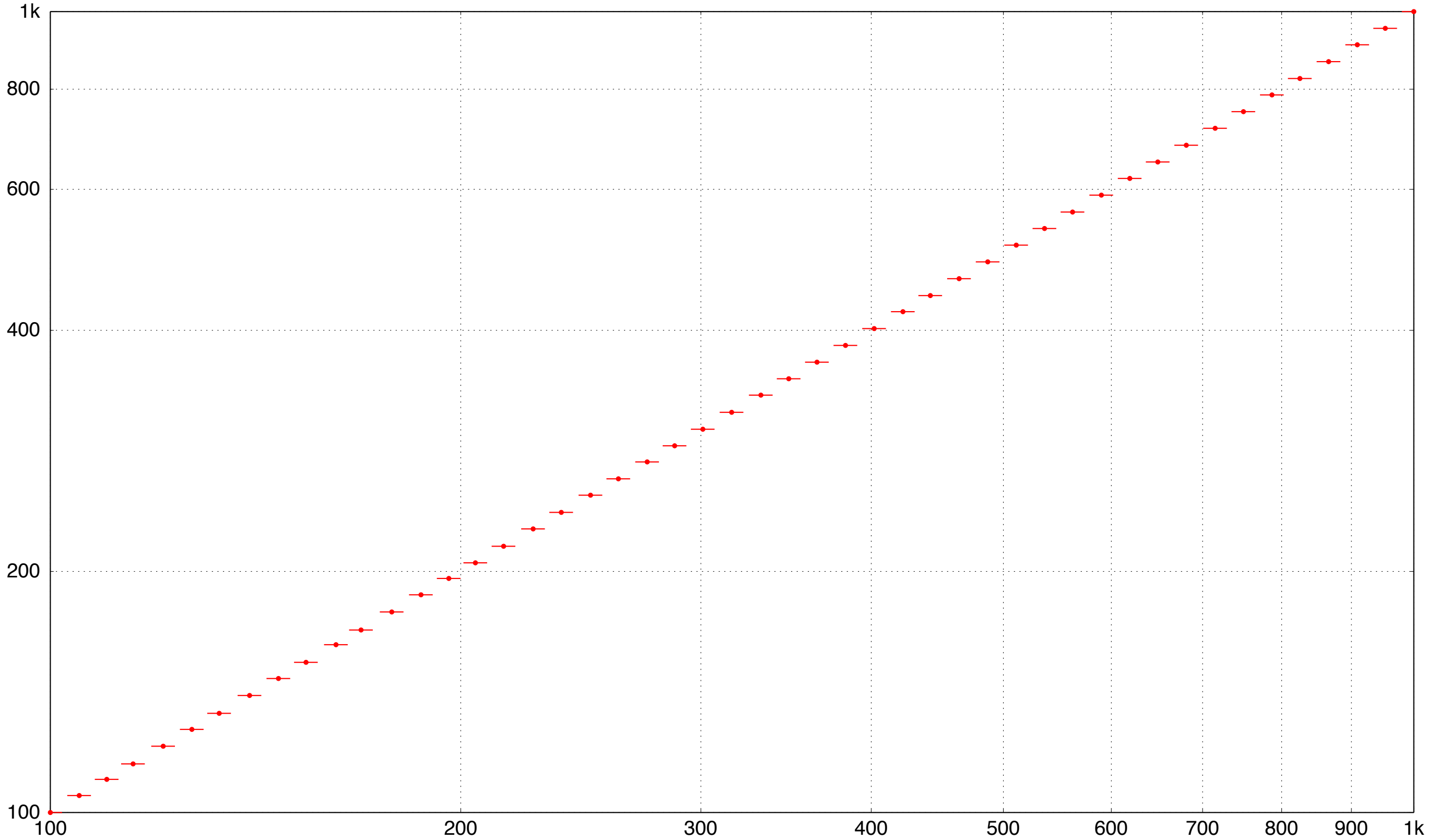
E48 series values between 100 and 1k with \pm 2\% tolerance bands
